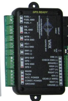
Control Box
